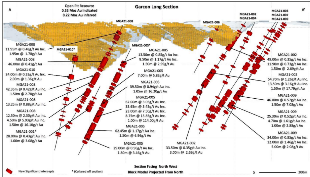
Figure 1: Cross Section showing high grade intervals below the Garrcon resource pits (Source: Moneta Gold Inc. Press release on Step-out drilling at Garrcon, Tower Gold Project, issued March 24, 2022)
